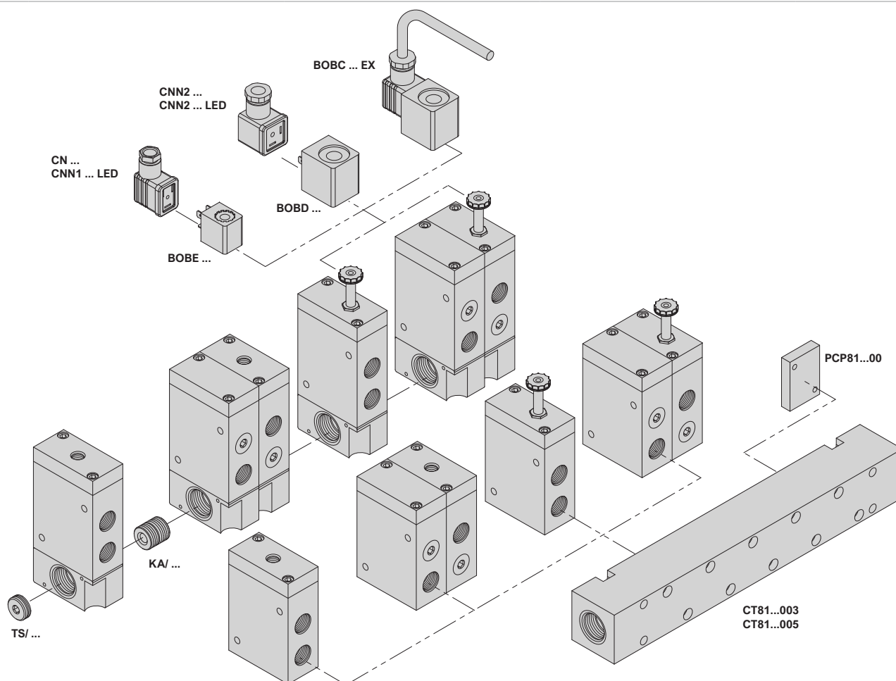
BOBE ... Coils type "E" AC / DC
